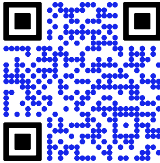
Twin Primes
