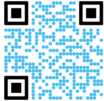
Fibonacci
